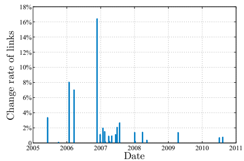
Figure 1: The rate of link changes between every two sampled successive commits for Axis2.java .
