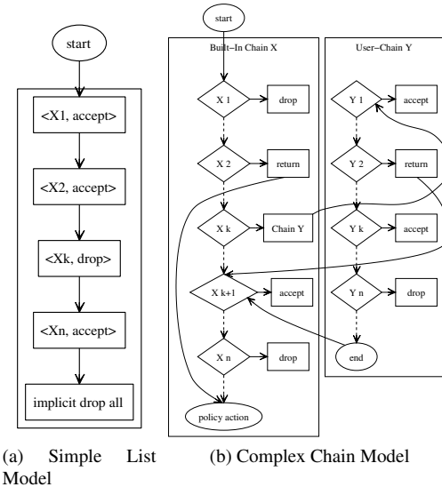
Figure 1: Model of individual firewalls.
