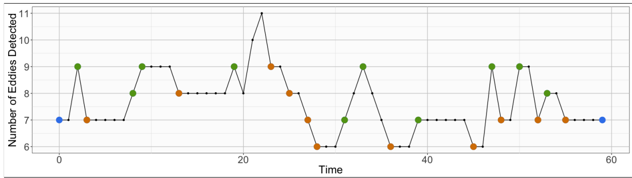
(a) B = 3, \alpha = 1, \delta^2 = 1, n_{flat} = 2
