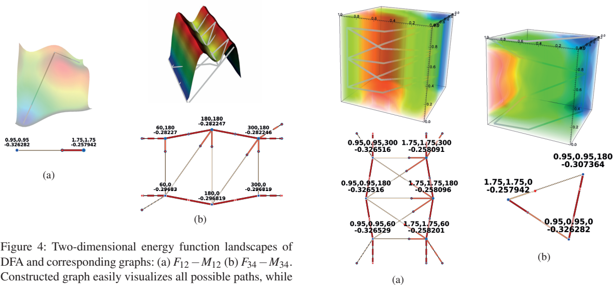
Figure 5: Three-dimensional energy function volume renderings of DFA and corresponding graphs: (a) F_{123} - M_{123} (b) F_{124} - M_{124} . As the number of dimensions grows, direct visualization becomes complicated.
