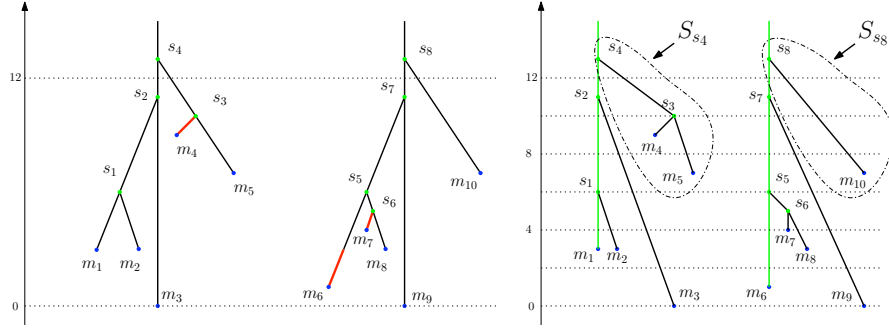
Fig. 5 Left: For the merge trees T_f, T_g , the smallest manually identifiable difference is shown as red segments. Right: The first iteration of the ISEPPSIMILAR function chooses (s_4, m_1) and (s_8, m_6) as root branches (depicted in green).
