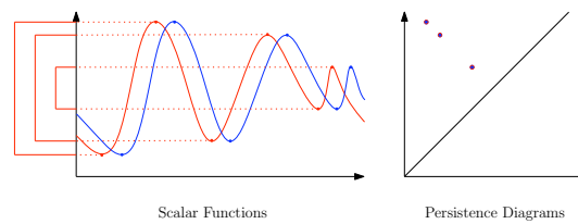
Fig. 1 Consider two scalar functions, where one is a slightly shifted version of the other. Comparing them directly, e.g., via the L_\infty norm, results in a large difference. Their persistence diagrams are the same, thus capturing the topological similarity of these functions.
