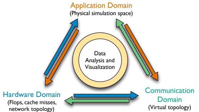
Fig. 2. The HAC model: Data used for performance analysis is divided into three domains. New visualization and analysis techniques that project data between these domains correlate problem symptoms in one domain to behavior in another, making it easier and more efficient to determine the problem origin.
