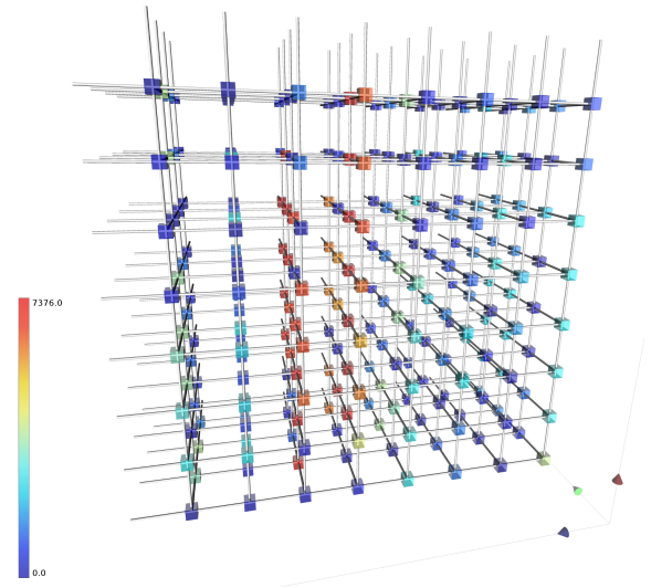
Fig. 8. Boxfish showing 256 nodes in a 8 \times 4 \times 8 torus colored by the time spent in phase 1 (load distribution) of load balancing. We observe processes in the third and fourth planes spend the most time in this phase and infer they are waiting. This grouping suggests examining the virtual tree topology used during load balancing.
