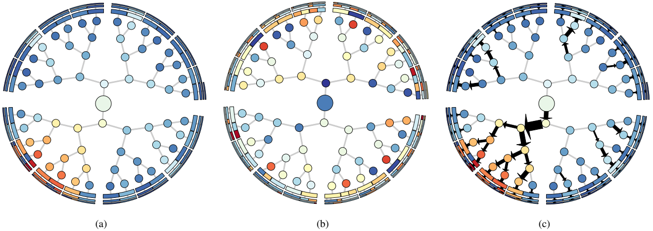
Fig. 9. Phase timing data and load information visualized in the communication domain, showing the virtual tree network of the load balancing phase (512 processes on Blue Gene/P). Nodes are aggregated at deeper levels and colored by their average weight. (a) Nodes colored by times spent waiting to receive excess load. (b) Nodes colored by the load before load balancing. (c) The tree of (a) with arrows scaled by the number of elements sent between nodes. This highlights the heavy use of few links which leads to increased wait times at the receiving nodes.
