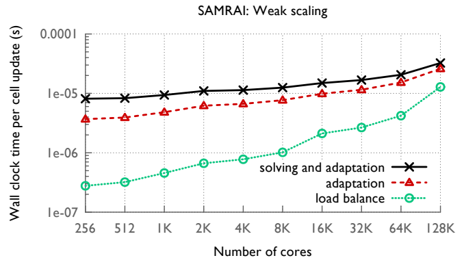
Fig. 4. Weak scaling performance of SAMRAI for the linear advection benchmark on Blue Gene/P. Mesh adaptation dominates for larger core counts where load balancing becomes problematic.
