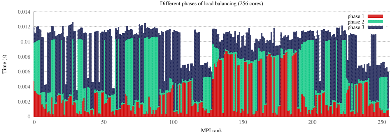
Fig. 7. Time spent in different load balancing sub-phases for 256 processes on Blue Gene/P. Some processes remain in phase 1 for a majority of time which is likely forcing others to wait. This observation is useful, but this graph does not scale to higher core counts and does not reveal the cause of the problem.
