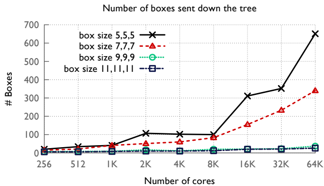
Fig. 15. Reduction in maximum number of boxes sent on any edge of the tree by increasing the size of each box.
