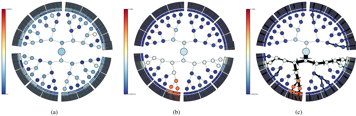
Fig. 1. Visualization of the binary tree shaped virtual communication topology used in SAMRAI's load balancing phase for 16,384 cores. Warmer colors (as one moves up the scale) represent higher values of load or time. (a) Nodes colored by load before load balancing: No imbalances are obvious. However, there are minor differences with the two top trees being slightly overloaded. (b) Nodes colored by times spent waiting to receive excess load. (c) The tree of (b) with arrows scaled by the number of boxes sent across, highlighting the problem. The tree structure of the SAMRAI load balancing scheme acts as a funnel with most excess being forced along a single edge causing a linear amount of processing.
