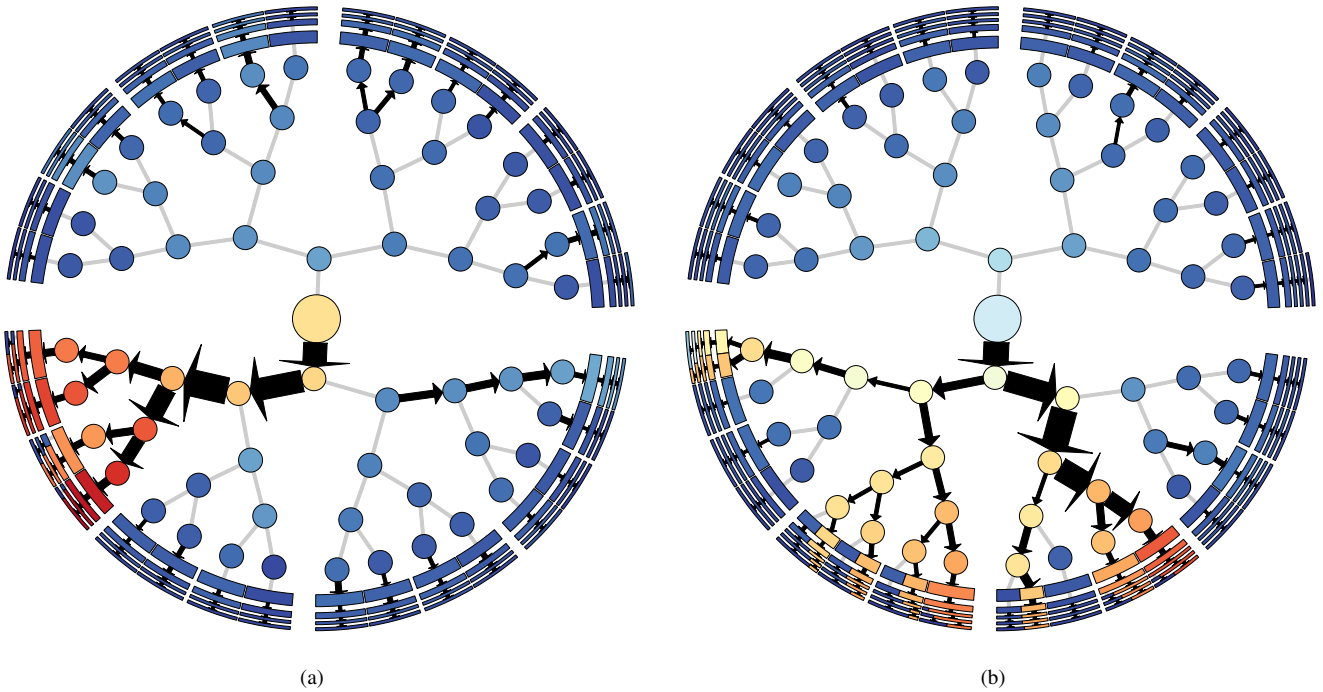
Fig. 11. The virtual binary tree topology colored by wait times in phase 1 of load balancing for (a) 1024 cores and (b) 2048 cores. Arrow weights are proportional to boxes sent between parent and child. As core counts increase, the load imbalance moves further down the tree and large numbers of boxes are routed through few edges, resulting in a flow problem.
