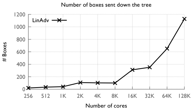
Fig. 10. Maximum number of boxes sent on any edge of the tree as a function of the number of cores (on Blue Gene/P). The virtual binary tree topology funnels a large portion of these messages through few links during load balancing causing the scalability bottleneck.
