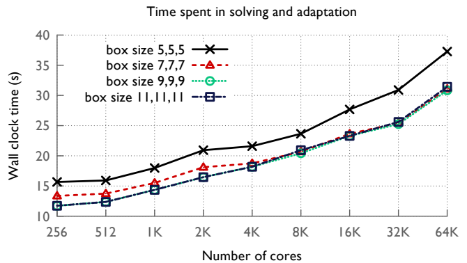
Fig. 17. Improvement in overall (solving plus adaptation) time by using larger, and thus creating fewer boxes.
