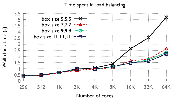
Fig. 16. Improvement in load balancing time by using larger, and thus creating fewer, boxes.
