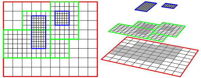
Fig. 3. A simple two-dimensional structured AMR mesh with three levels of refinement (left). The same mesh is shown as a hierarchy on the right. Cells that are refined are shown in gray.
