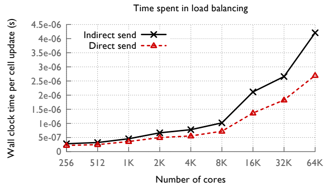
Fig. 14. Reduction in load balancing time by sending patches directly to their new destinations rather than through the binary tree.
