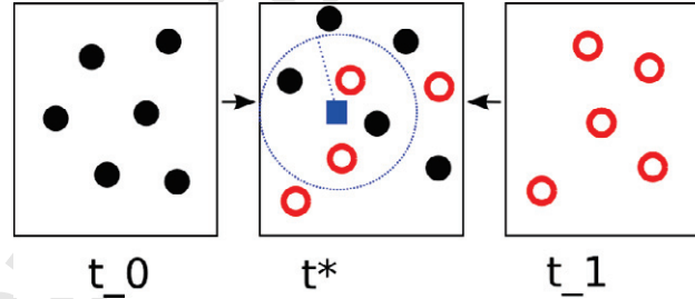
Figure 1: Proposed interpolation scheme: Forward advection of fluid particles from previous time-step to intermediate stage t^* , and recalculation of the velocity field. Backward advection of fluid particles from the last time step, recalculation of the velocity field. Data is re-sampled at intermediate time t^* at blue points using a radial basis function.
