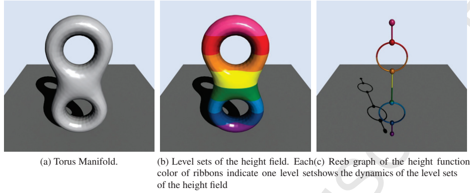
Figure 6: A double torus example of Reeb graph
