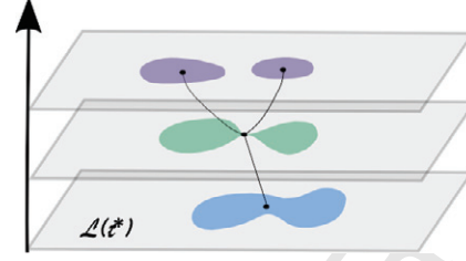
Figure 5: Level sets of a function and its' Reeb graph.
