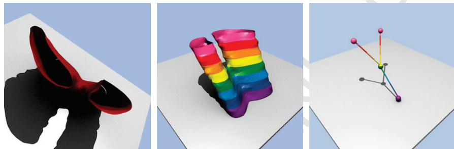
(a) Bifurcation: regions splittings after a certain time point. Outer normal of the plane points to time direction
