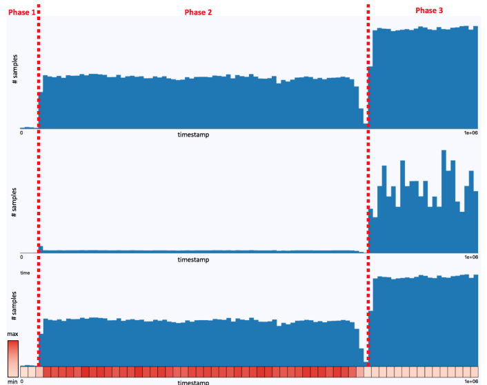
Fig. 12: Top: single histogram of time dimension, where three time sections can be seen, indicating different execution phases (marked). Middle: same dimension after selecting accesses to NUMA resources; nearly all NUMA accesses occurred during the third phase. Bottom: same dimension with L2 imbalance metric shown along the axis. It can be seen and concluded that the second phase caused the most L2 cache imbalance, relatively.
