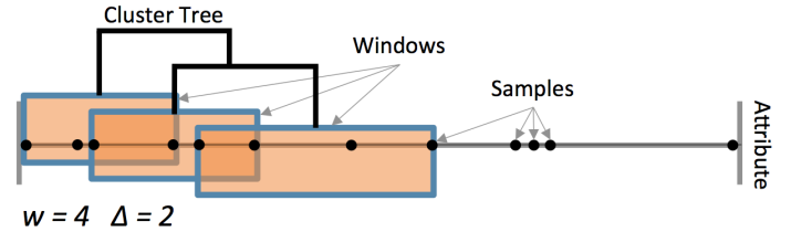
Fig. 7: The process for clustering memory access samples. We create a window with w samples starting with the minimum value along the attribute and move it by an amount \Delta < w samples until we reach the end, creating a subset for each set of w samples within each window position. We agglomeratively cluster the subsets using our proposed metrics in Section 7 as distance metrics.
