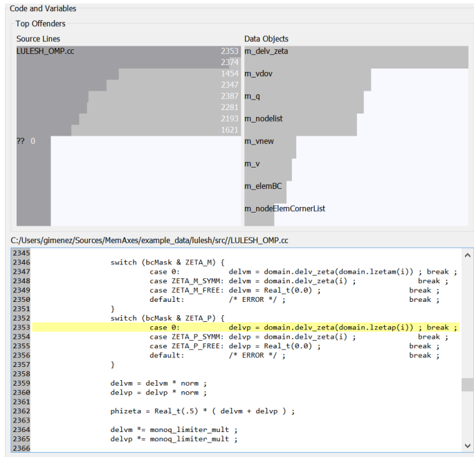
Fig. 2: Visualization of memory access data in the context of the top offending lines of source code (top left) and data objects (top right). The topmost offending line of source code is shown highlighted within its containing file in the source pane (bottom).
