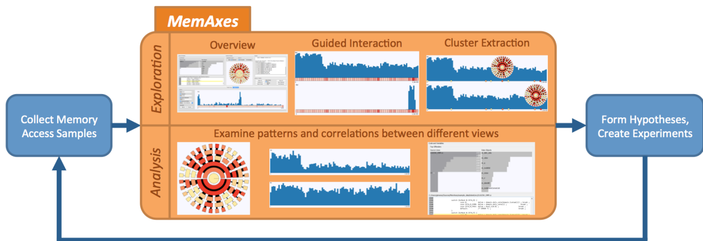
Fig. 1: Exploration and analysis workflow for characterizing memory performance using MemAxes. Initially, MemAxes shows the overview of all memory access samples, then through guided interaction and cluster extraction the user may select regions of interest. On any selection of data, the analyst may draw conclusions by identifying patterns in different views and seeing how patterns between multiple attributed contexts correlate with one another.
