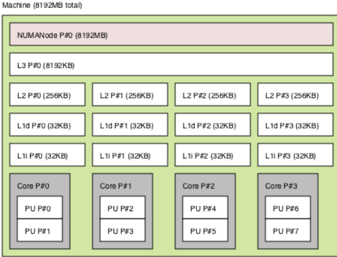
Fig. 3: The hardware topology visualization produced by hwloc , which uses a horizontal layout. The pink rectangle denotes a single RAM resource [5]. The caches are drawn underneath in white, processor cores dark gray, and processing units (CPUs) embedded inside the cores.
