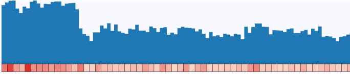
Fig. 6: Histogram and guided interaction along a single attribute. The colored rectangles on the bottom encode derived metrics for bins of samples along the attribute. Darker colors indicate areas of higher imbalance across NUMA memory resources.
