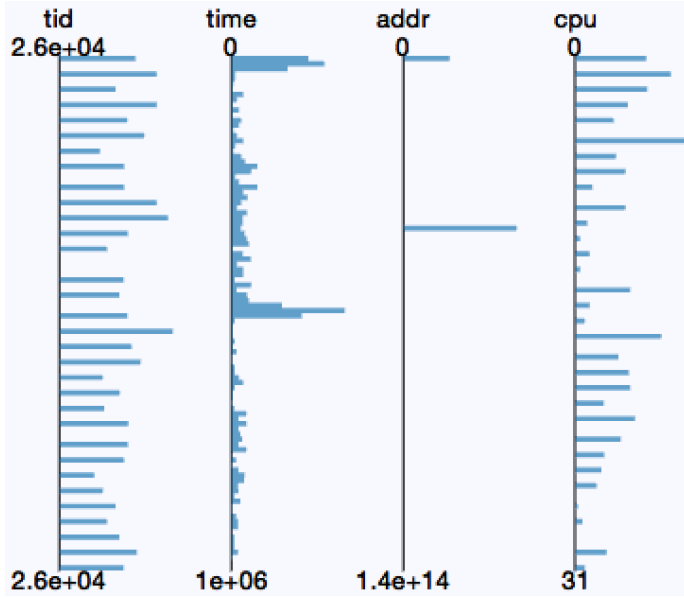
Fig. 5: Parallel histograms of memory access samples. Each attribute is plotted along a vertical histogram and all attribute histograms are placed side-by-side in parallel.
