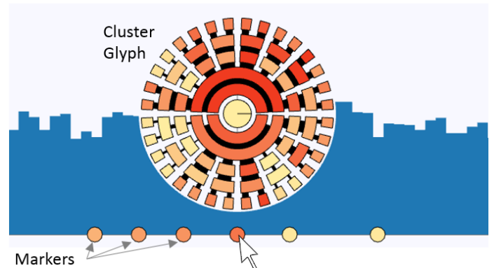
Fig. 8: Cluster viewing and selection. Clusters of a specified depth and metric are shown along the attribute's axis as markers (circles) colored by their derived metrics. When the user hovers the mouse pointer over a marker, a glyph expands showing the hardware topology visualization for the subset of samples contained in the cluster. Upon clicking the marker, the subset is selected for further analysis.
