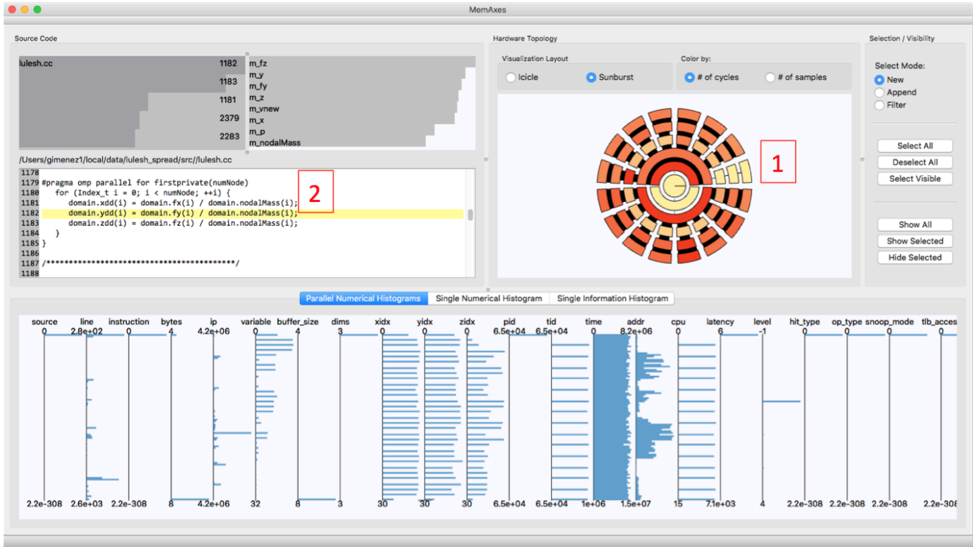
Fig. 9: MemAxes upon opening the memory performance data collected from LULESH, before performing any interaction. In the topology view (marked 1) we can see one processor was extremely under-utilized relative to the rest. We also see that several accesses were made to the top NUMA node (the dark orange arc directly above the center) but few if any were made to the bottom one. In the code/data view (marked 2) we see a parallel loop in the code accessing elements fy and nodalMass from the domain. In the top offenders view directly above, we see more time was spent waiting for fy than nodalMass .
