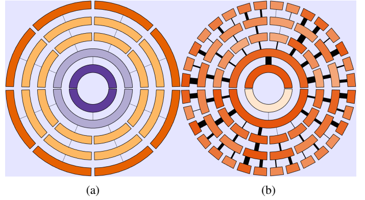
Fig. 4: (a) The radial layout of the hardware topology in MemAxes for a simple architecture. Main memory resources are dark purple, L3 caches are light purple, L1 and L2 caches are light orange, and processing units are dark orange. (b) A more complex architecture with performance data annotated onto the hardware resources, via a color map, and transactions between them, via a line width.
