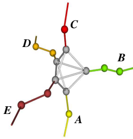
Fig. 7. The interior (colored) points of ascending 1-manifolds A , B , C , D , and E meet at a cluster of vertices (grey). This set denotes a maximum node in the complex, since it forms the boundary between the ascending 1-manifolds. The selection of the maximum vertex within A_0 associated with A , B , C , D , and E does not change the topology of the complex. We pick the highest vertex in the cluster for which all the ascending 1-manifolds are incident.
