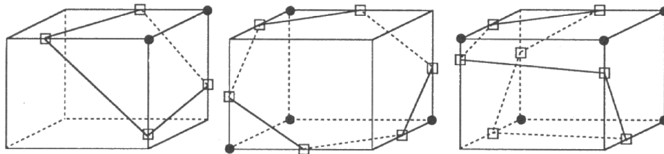
Figure 5. — Possible contour polygons inside cubes.
