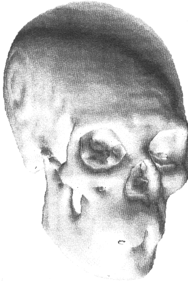
Figure 8. — Human skull as contour of a density function.
