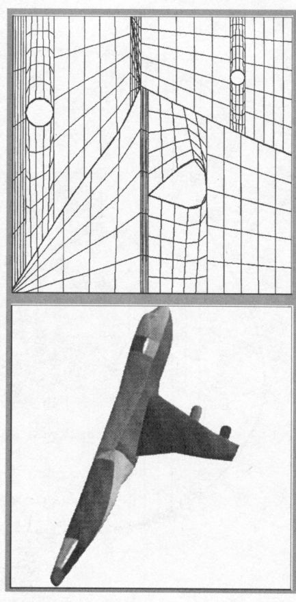
Fig. 11. Fuselage with multiple trimming curves.
