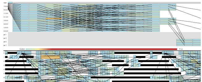
Figure 15: Differential duration on a 16-chare execution of Jacobi 2D. One chare experiences a significantly longer compute time (orange).
