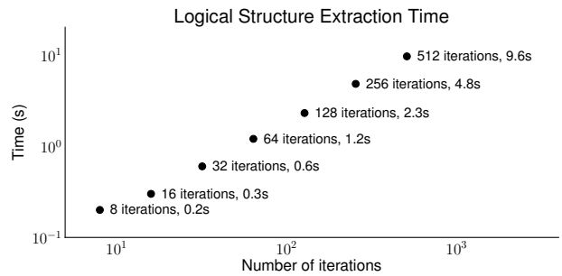
Figure 18: Time to calculate logical structure for a 64-chare LULESH execution at increasing iterations.
