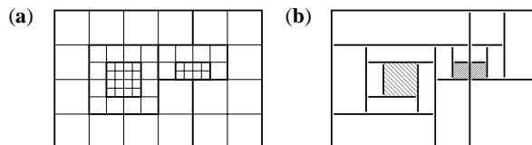
Figure 2: Homogenizing a 2D AMR hierarchy. The hierarchy has a uniform refinement ratio of two. Grid boundaries are denoted by bold lines. All hierarchy levels consist of two grids. Note that finer grids can cross boundaries between coarser grids. (a) Original AMR hierarchy with overlapping grids. (b) Homogenized hierarchy with non-overlapping rectangular grid patches.
