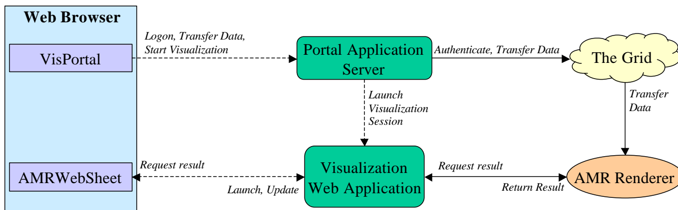
Figure 2: The VisPortal/AMRWebSheet architecture. Elements within the blue box represent web pages that the user interacts with, green boxes represent web servers, and the other nodes represent grid-accessible resources. Dashed lines are HTTP/HTTPS connections for HTML and images (for the client) and connection requests (for the server), and solid lines are TCP connections. A line's label indicates the action performed over that link; for bidirectional connections, the top label corresponds to actions initiated from the left entity while the bottom label corresponds to actions initiated from the right entity. Note that the AMR renderer can be located anywhere on the Grid—the VisPortal initializes the connection between the renderer and the visualization web application when a visualization is first requested.
