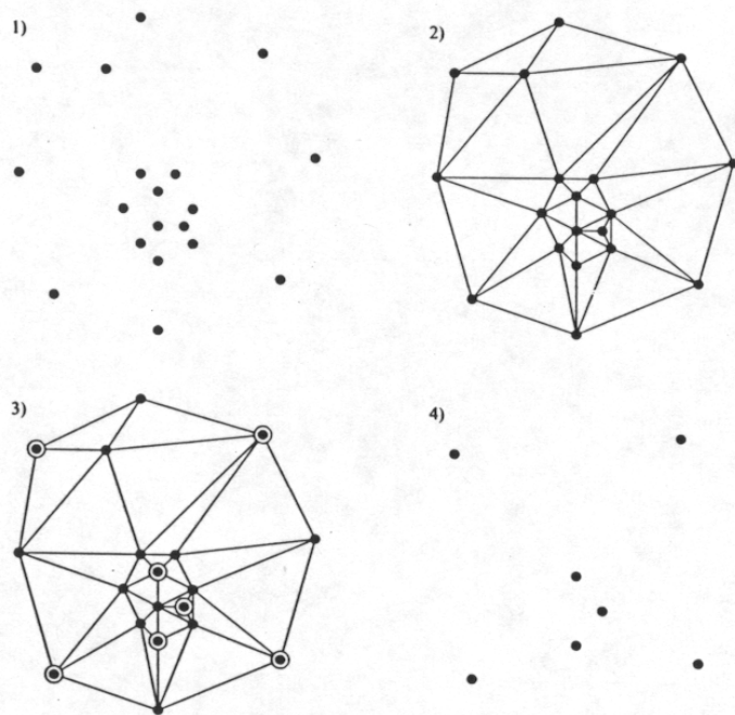
Figure 7: Creating a lower-resolution approximation of a point set by extracting the maximum independent set. 1) The original point set; 2) the original set’s Delaunay triangulation; 3) the point set’s maximum independent set (included points are circled); 4) the decimated point set.
