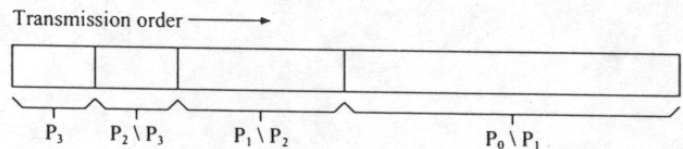
Figure 8: Storing a four-level approximation hierarchy in a file. The coarsest-resolution level P_3 is stored first.
