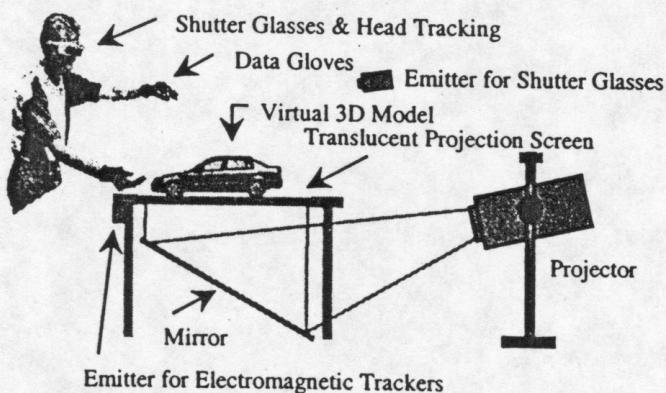
Figure 2: Hardware setup
