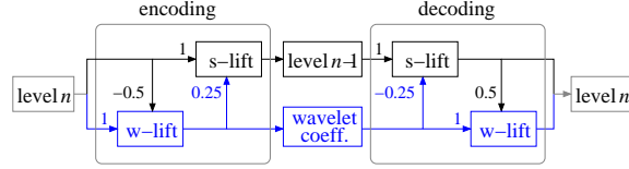
Figure 4: One-dimensional linear B-spline wavelet lifting scheme.
