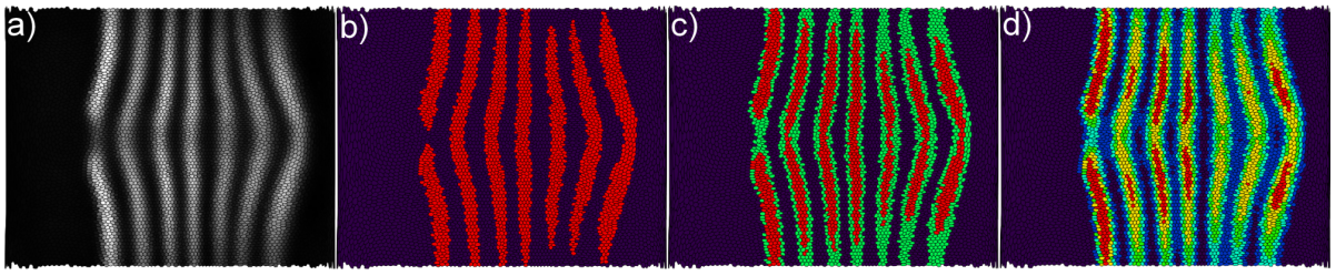
Fig. 9. a) The expression pattern of eve at stage 5:9-25%; Classification of eve with b) k = 2 ; c) k = 3 ; and d) k = 6 . While the k = 2 clustering produced a threshold that was too high, erasing too many cells from the pattern, the k = 3 clustering was better able to identify the seven stripes of the eve expression pattern. The k = 6 clustering identified additional characteristic variations within the stripes along the DV-axis as well as an additional cluster that selects some inter-stripe cells showing some higher expression of eve .
