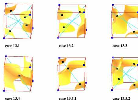
Figure 7: Topological configurations with six ambiguous faces: trilinear model in yellow-orange, isopoints in black, positive nodes in blue, rays in cyan.
