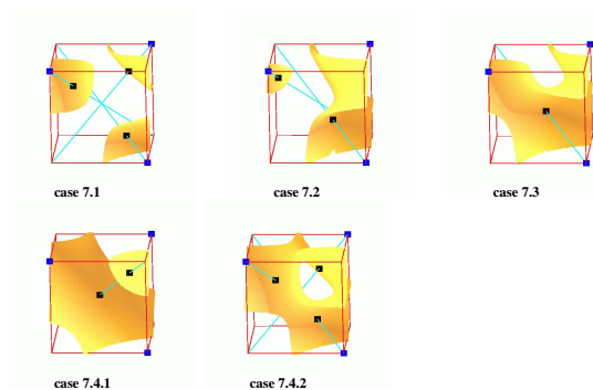
Figure 6: Topological configurations with three ambiguous faces: trilinear model in yellow-orange, isopoints in black, positive nodes in blue, rays in cyan.
