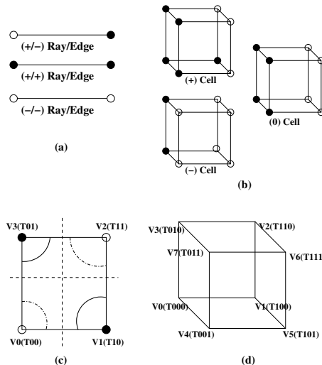
Figure 2: (a) Sign of ray/edge (b) Sign of cell (c) Ambiguous face with the notations used for vertices and their scalar values in bilinear interpolation. Solid contours occur when the face is separated with respect to positive sign, and dotted contours occur when with respect to negative sign (d) Notation for cell vertices for trilinear interpolation. Black and white vertices are positive and negative, respectively.
