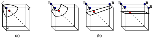
Figure 8: (a) Associations of isosurface point (in red) with vertex A (in blue), which is the endpoint of the intersecting diagonal closer to the isosurface (curved lines), and the edges “e” containing A; (b) Configurations where isosurface point is associated with vertex A on the intersecting diagonal, and additional associations between isosurface point and vertices, B, are made. Blue cell vertices are associated with the red isosurface point, the bold dotted line is the intersecting diagonal, and the curved boundary is the isosurface.
