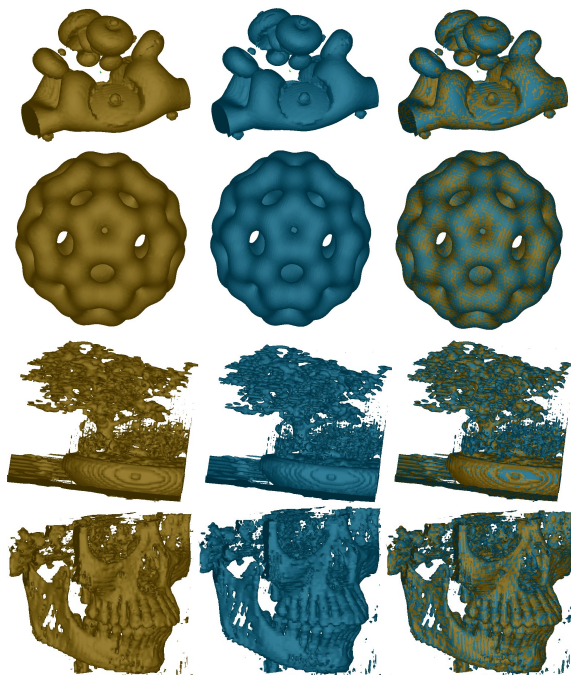
Figure 9: Dual contouring result (left), MC result (middle), and comparisons of both surfaces by superposition for regular datasets of size 64x64x64 of Neghip (top) and Buckyball (second), and of size 256x256x256 (rendered in 1:4) of Bonsai (third) and Skull (bottom). (Datasets available at http://www.volvis.org .)
