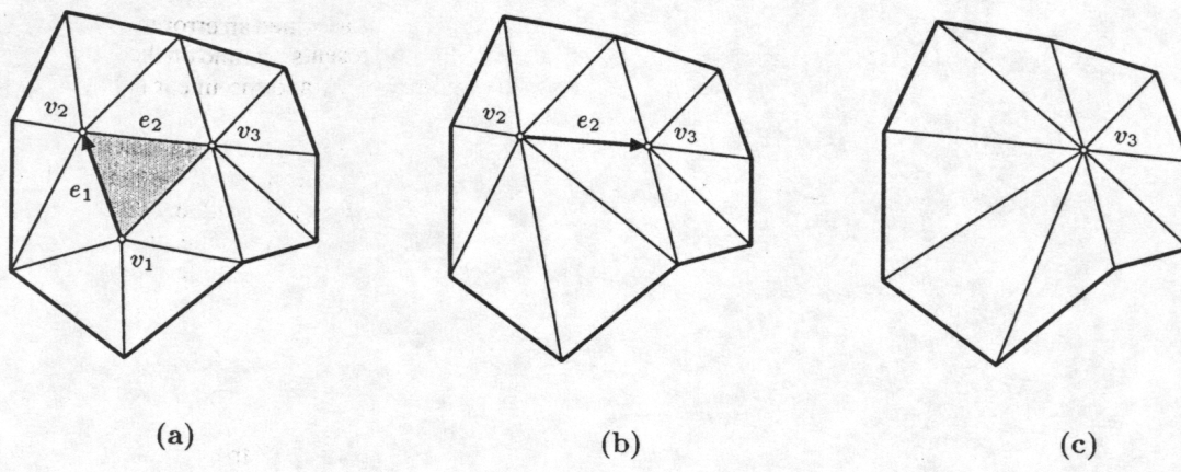
Figure 2: A two-edge collapse of a triangle T : (a) the triangle and its associated stencil; (b) the mesh after the collapse of edge e_1 ; (c) the mesh after the collapse of both e_1 and e_2 .
