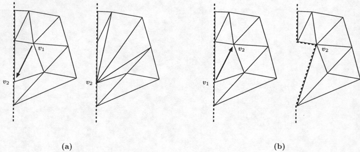
Figure 6: Collapsing edges on the boundary: (a) an edge is collapsed to a boundary vertex; (b) the boundary is destroyed when the collapse goes the other way.
