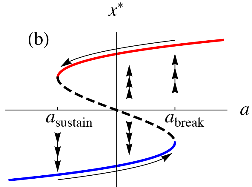
Cusp bifurcation/catastrophe
