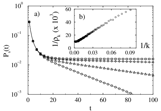
FIG. 3. (a) Surviving probability P_s(t) for a spreading rate \lambda = 0.065 in scale-free networks of size N = 5 \times 10^5 ( \square ), N = 2.5 \times 10^4 ( \diamond ), N = 1.25 \times 10^4 ( \triangle ), and N = 6.25 \times 10^3 ( \circ ). The exponential behavior, following a sharp initial drop, is compatible with the data analysis of Fig. 1. (b) Relative density \rho_k versus k^{-1} in a SF network of size N = 5 \times 10^5 and spreading rate \lambda = 0.1 . The plot recovers the form predicted in Eq. (2).
