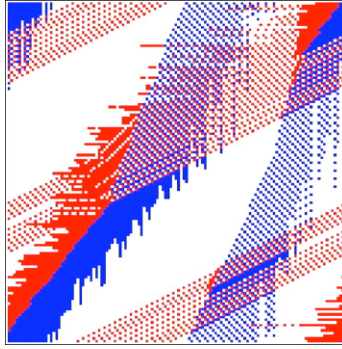
Fig. 7. A typical PI state on a square lattice for a realization with L = L' = 128 and \rho = 0.36 . System 2 of Ref. [10] illustrates the dynamics.
