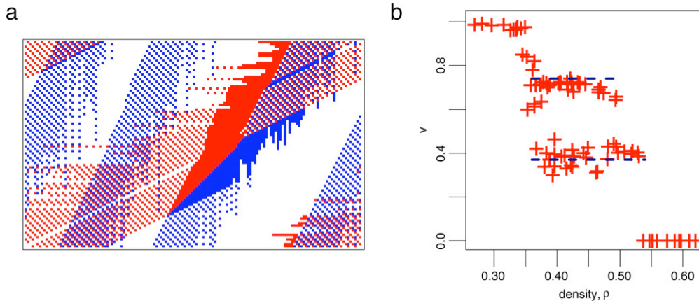
Fig. 2. (a) Typical PI state on a Fibonacci lattice for a realization with L = 144 and L' = 89 . (b) Experimental results for L = 89 and L' = 55 . Each point represents one individual realization. For densities between \rho \approx 0.35 and \rho \approx 0.5 , each realization converges to a PI state.
