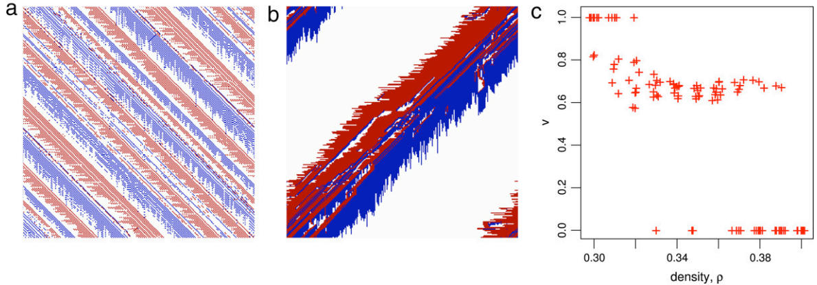
Fig. 1. Typical configurations for the BML model on an L \times L lattice, with L = 256 . (a) The free-flow (FF) phase reached by any random initial configuration with small density, \rho . Self-organized bands of separated east-bound and north-bound cars allow all particles to advance each update, thus v = 1 . (b) The global jam (GJ) phase reached by any random initial configuration for larger \rho . Here all cars are immobilized, thus v = 0 . The conventional belief is that there is a first-order phase transition between these two behaviors as a function of \rho , with critical density \rho_c \approx 0.35 . (c) Numerical results show otherwise. Each point represents one individual random realization run until convergence. FF ( v = 1 ) and GJ ( v = 0 ) states do occur, but less frequently than intermediate states.
