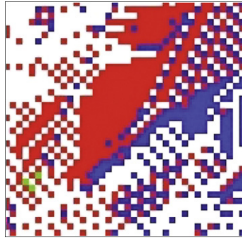
Fig. 8. Closeup of the DI state shown in Fig. 3, with L = L' = 128 and \rho = 0.36 . Perturbing just three particles (colored green, lower left hand corner), will make the new system converge to GJ. (System 4 of Ref. [10] is a movie of the dynamics, started from the perturbation.). (For interpretation of the references to colour in this figure legend, the reader is referred to the web version of this article.)
