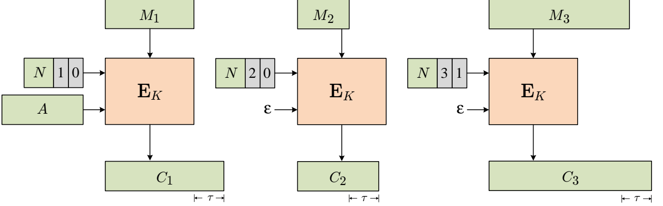
Fig. 8: The STREAM construction for nOAE. Encryption scheme \Pi = (\mathbf{K}, \mathbf{E}, \mathbf{D}) secure as an nAE with ciphertext expansion \tau is turned into a segmented-AE scheme \Pi' = (\mathcal{K}, \mathcal{E}, \mathcal{D}) = \mathbf{STREAM}[\Pi, \langle \cdot \rangle] with key space \mathcal{K} = \mathbf{K} .
