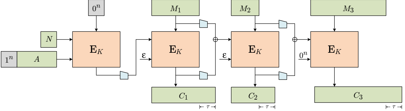
Fig. 7: The CHAIN construction for OAE2. Top: Encryption scheme \Pi = (\mathbf{K}, \mathbf{E}, \mathbf{D}) , secure as a PRI with expansion \tau , is turned into a segmented-AE scheme \mathbf{CHAIN}[\Pi, n] = (\mathcal{K}, \mathcal{E}, \mathcal{D}) with \mathcal{K} = \mathbf{K} . Bottom: Illustration of segmented encryption where each segment of (M_1, M_2, M_3) has at least n bits. The trapezoid represents truncation to n bits.
