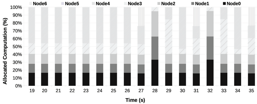
Fig. 5. Assignment of computation work during the simulation
