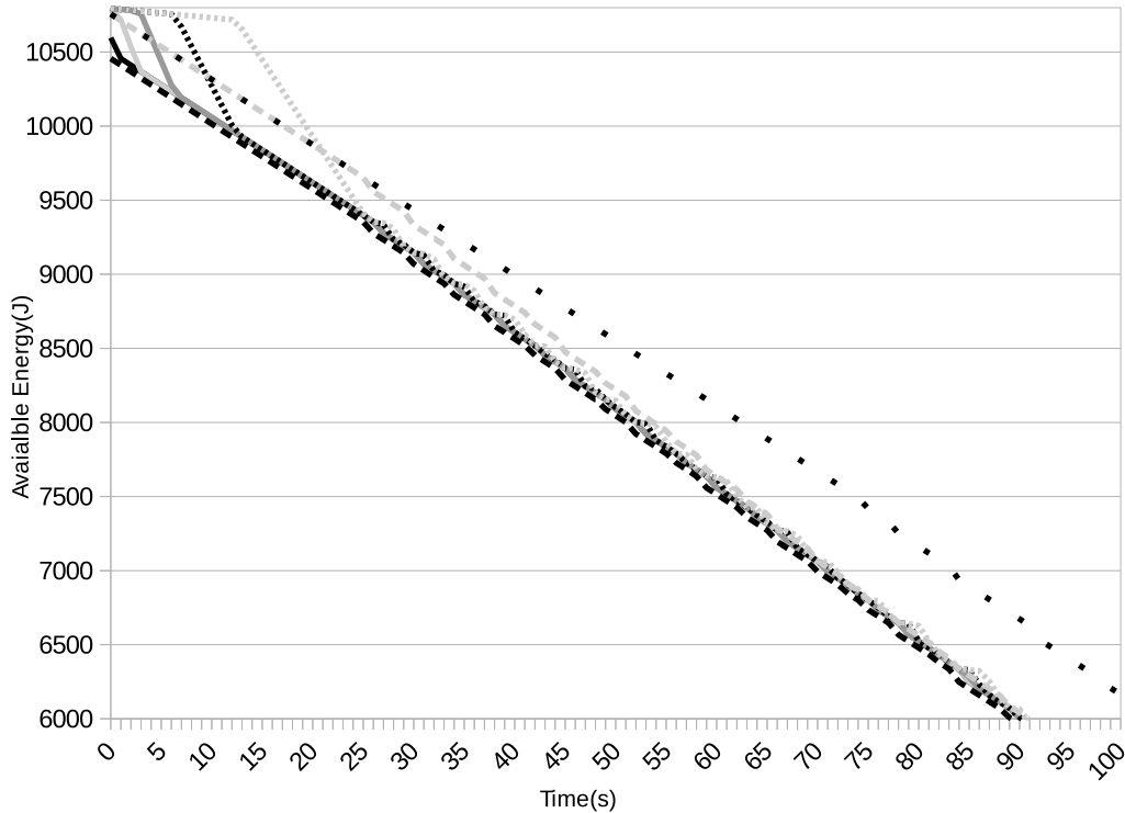
Fig. 6. Available energy on nodes during MME simulation [Time 0s-100s]
