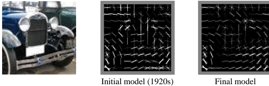
Fig. 5 Visualization of the positive HOG weights learned for the discovered frontal car visual element. Compared to the initial model, which was trained on the 1920s images, the final model cares much less about the car’s global shape but still prefers see a wheel in the lower-left corner.
