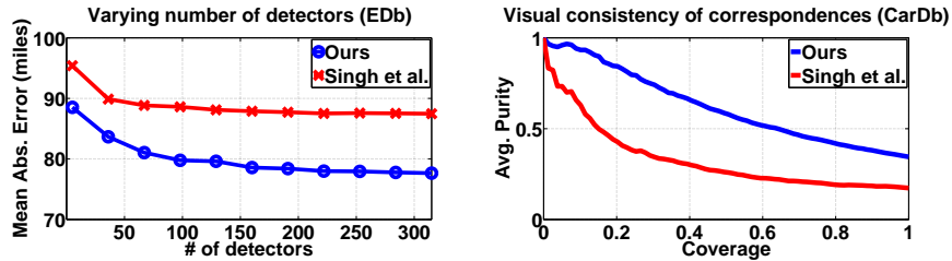
Fig. 10 Absolute prediction error rates when varying the number of detectors (lower is better), and visual consistency of correspondences measured using purity and coverage (higher is better).
