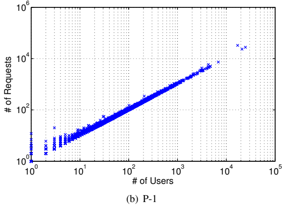
Fig. 13. Repeated access of objects
