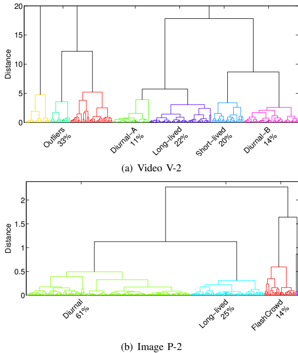
Fig. 8. Content clustering dendrograms of two adult websites.
