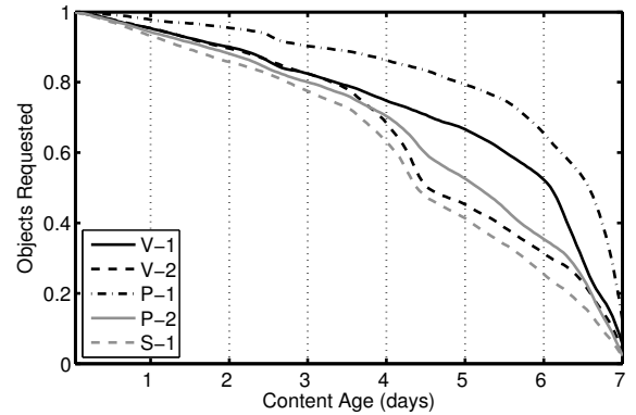
Fig. 7. Fraction of total object requested for adult websites at different ages
