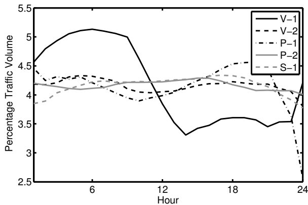
Fig. 3. Hourly traffic volume timeseries of five adult websites.
