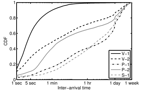
Fig. 11. User request inter-arrival time distributions
