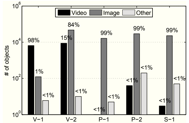
Fig. 1. Content composition of five adult websites. V-1 uses 6.6K objects, V-2 uses 55.6K objects, P-1 uses 16.3K objects, P-2 uses 29.6K objects, and S-1 uses 22.9K objects. We breakdown content into 3 categories: (1) video, (2) image, and (3) other. Other category includes objects that are not classified as video or image.
