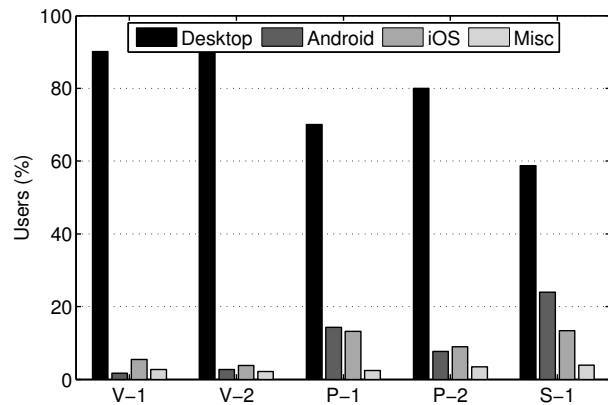
Fig. 4. Device type composition
