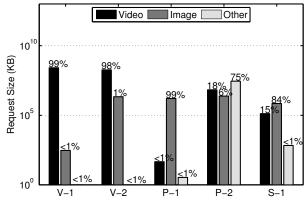
(b) Request Size
