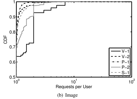
Fig. 14. CDF of repeated content access by users
