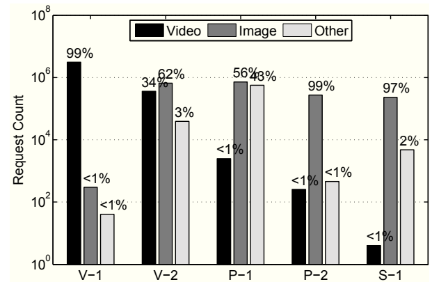
(a) Request Count
