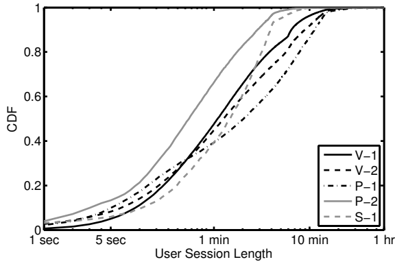
Fig. 12. User session length distributions
