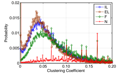
Fig. 7. Distribution of clustering coefficient
